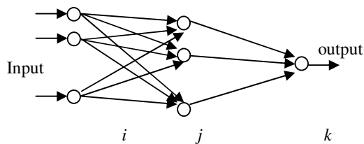
Gambar 5. ANNPSO Biclass topology
