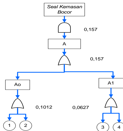
Gambar 8 Probabilitas Seal Kemasan Bocor
